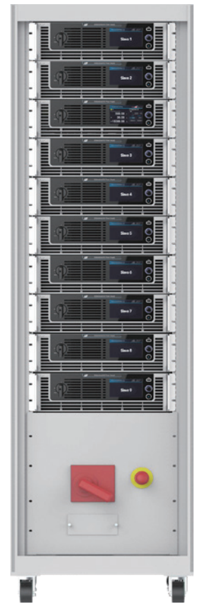
Master/slave parallel operation up to 180kW * Call for availability
